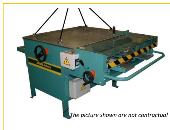
Standing seam shaping machine
